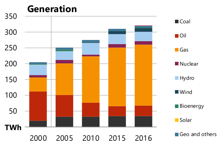
Figure 1: Mexico's power generation, 2000-16
