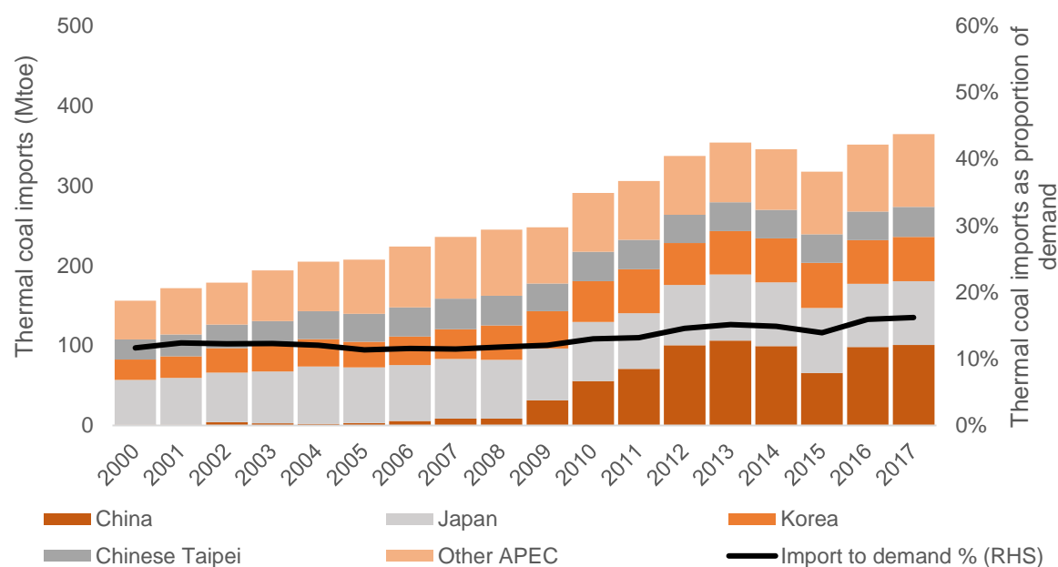
Figure 1.20: Thermal coal imports and proportion of thermal coal imports to thermal coal demand, APEC economies, 2000–2017
